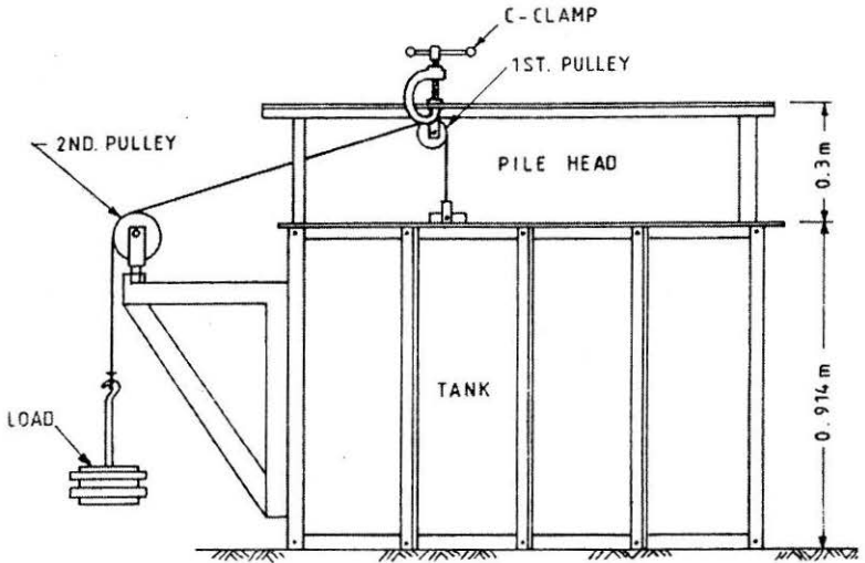
FIGURE 18 : Schematic Diagram of Experimental Assembly (Patra, 2001)
