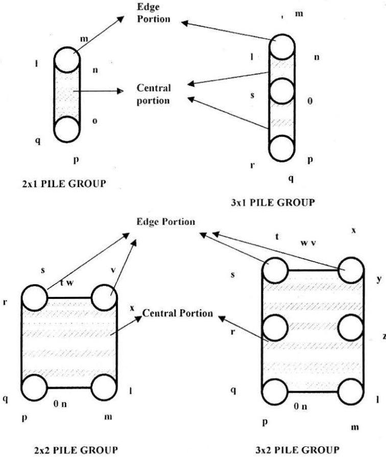
FIGURE 20 : Schematic Diagram of Pile Groups Showing Different Zones (Patra, 2001)
