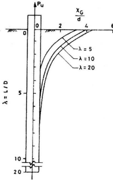
FIGURE 15 : Failure Surface for Different Slenderness Ratios ( \phi = 40^\circ, \delta = 10^\circ ) (Chattopadhyay and Pise, 1986)
