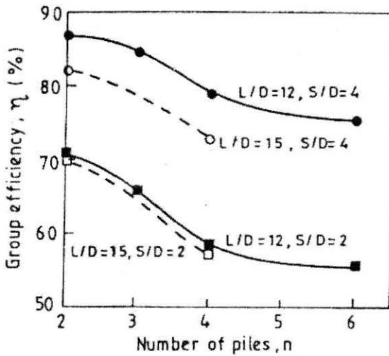
FIGURE 10 : Variation of Group Efficiency with No. of Piles in the Group and S/D (Das and Azim, 1985)
