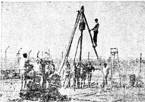
FIGURE 4 Driving operation for installation of rope drains.
