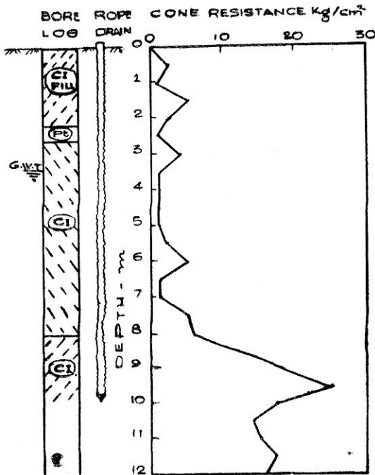
FIGURE 3 Borelog and static core resistance.
