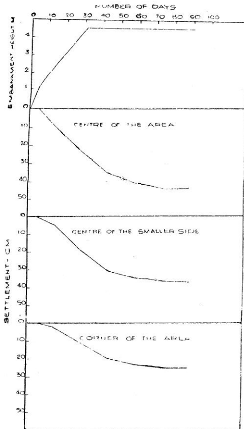
FIGURE 5 Programs of loading and settlement of ground
