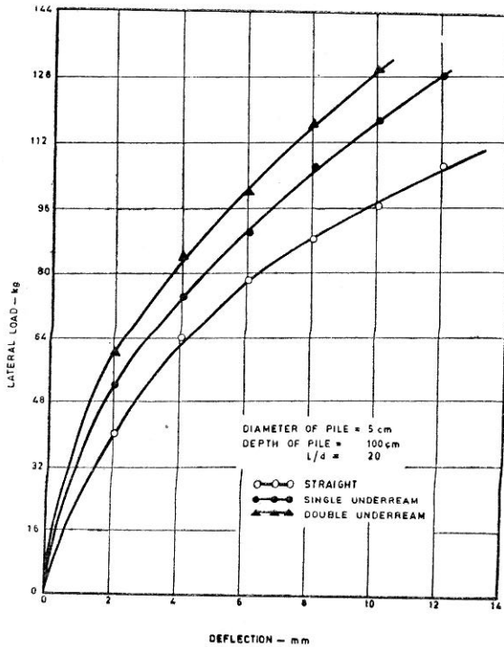
FIGURE 14 Effect number of bulbs in piles ( L/D = 20 )
