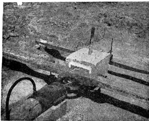
FIGURE 7 Lateral load test set-up in field
