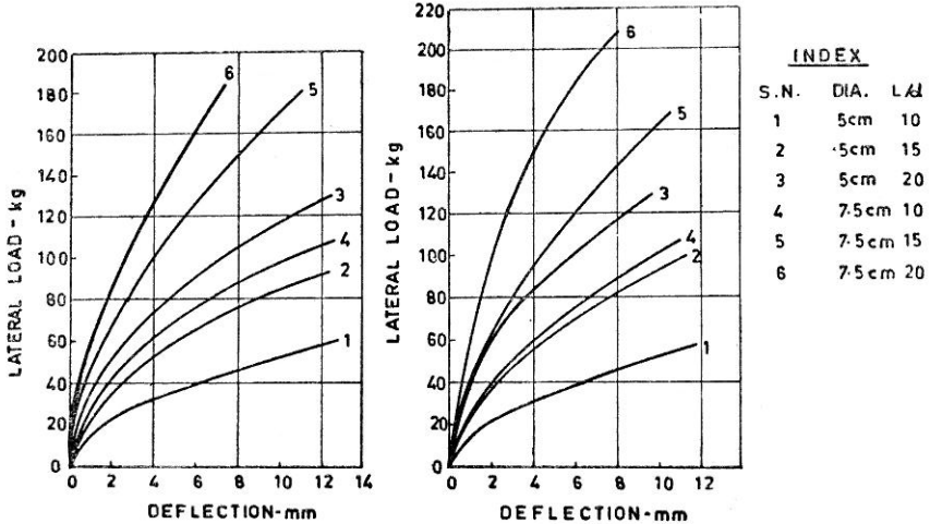
FIGURE 9 Effect of depth in single underream pile
