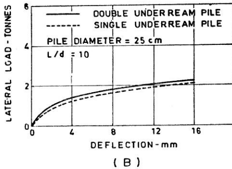
FIGURE 15 Effect of Number of bulbs in piles
