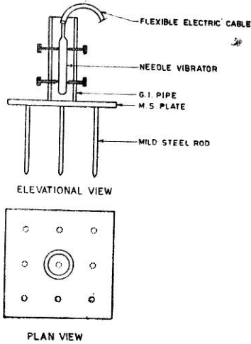
FIGURE 3 Apparatus for vibrating sand (not to the scale)
