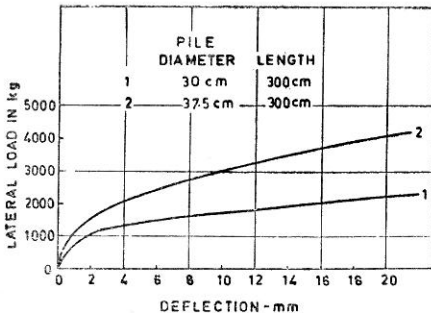
FIGURE 17 Effect of Shaft diameter of pile on its lateral load capacity
