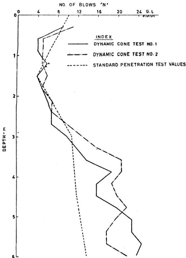
FIGURE 5 Penetration test results
