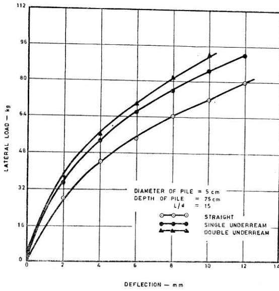
FIGURE 13 Effect of number of bulbs in piles ( L/D = 15 )
