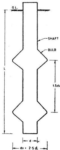
FIGURE 1 Under-ream pile
