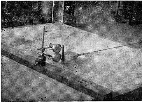
FIGURE 6 Lateral load test set-up in model
